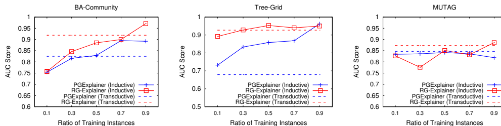
Figure 2: Comparison between RG-Explainer and PGExplainer in the inductive setting.
